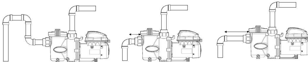
Incorrect: Air retention and risk of incorrect pre-filter filling.
